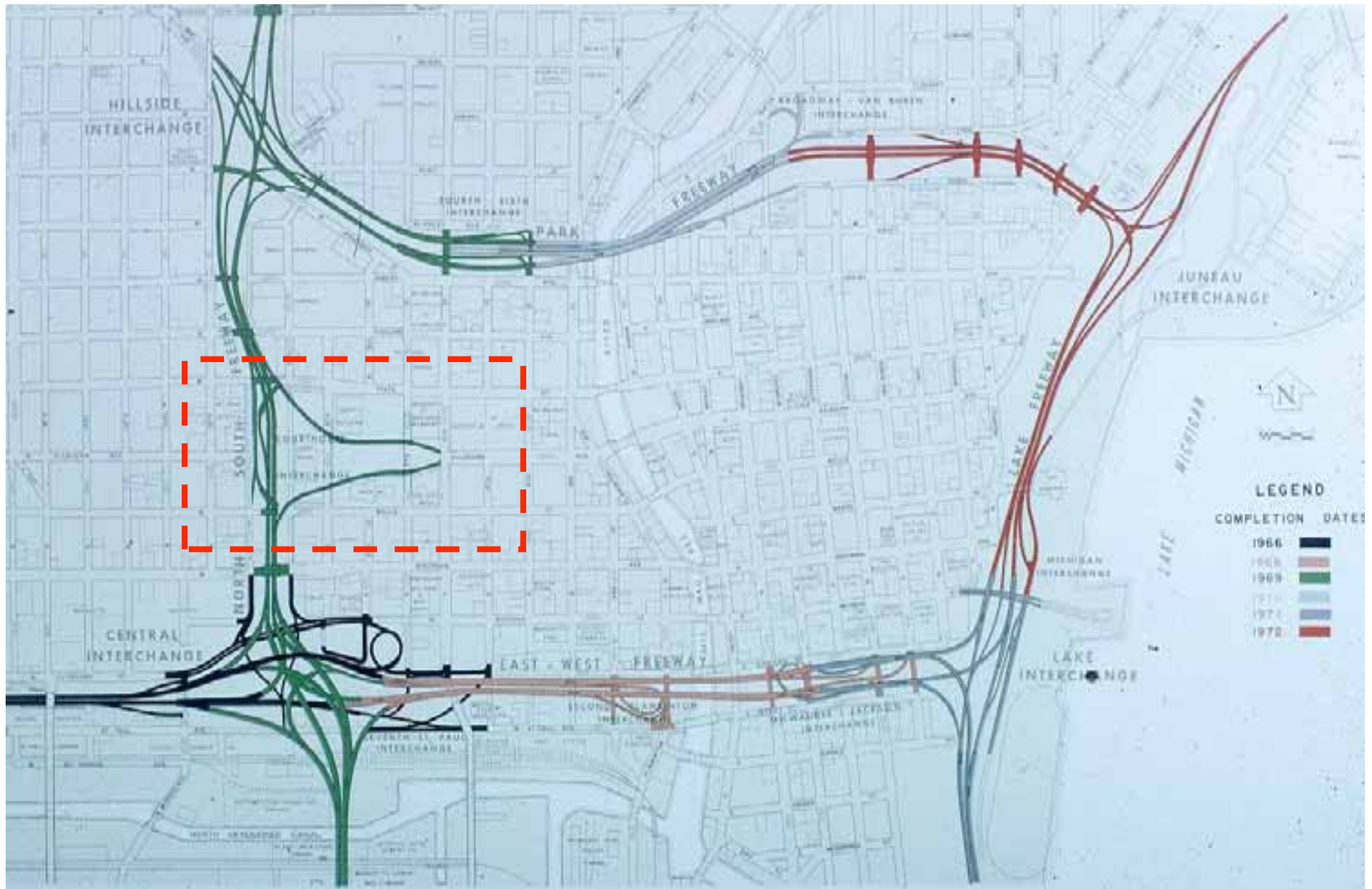
Figure 9 - Downtown Freeway Loop: Completion Schedule
